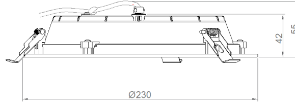
Cut-out : Ø215mm
